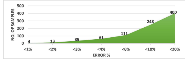
Figure 8: Error distribution for 400 data samples on ARM.
