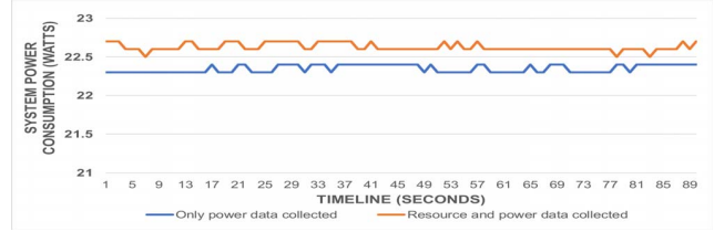
Figure 4: Data collection overhead for 89 seconds on Intel Xeon.
