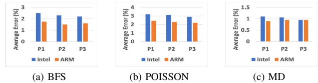
Figure 13: Average power estimation error (%) for different input configurations of benchmarks on a single container.
