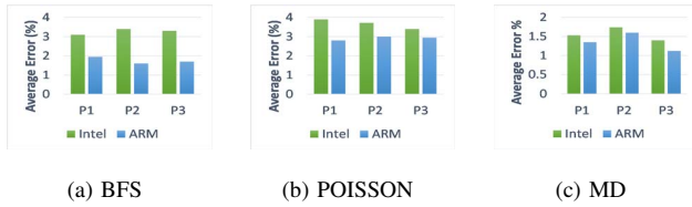
Figure 14: Average power estimation error (%) for different input configurations of benchmarks across two containers.
