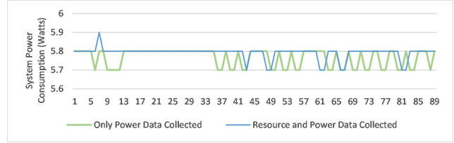
Figure 5: Data collection overhead for 89 seconds on ARM.
