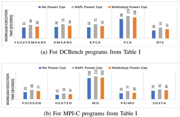
Figure 15: Execution time when a single container executes using the power cap technique on Intel Xeon.
