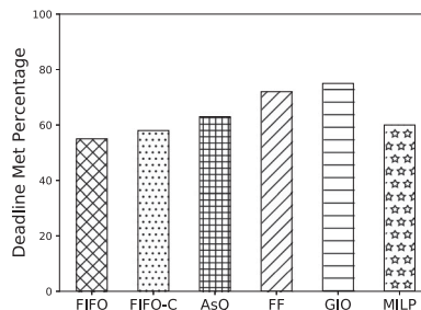
Fig. 9. Comparison of deadline met percentage between the scheduling algorithms (the higher the better).
