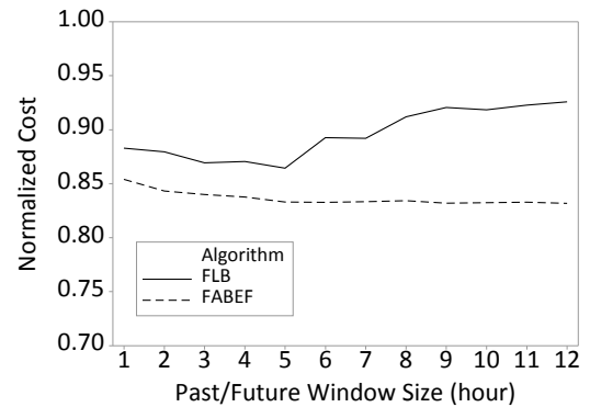
Fig. 12. Effect of window size on the total cost performance of FLB and FABEF normalized to the outcome of the RR algorithm.
