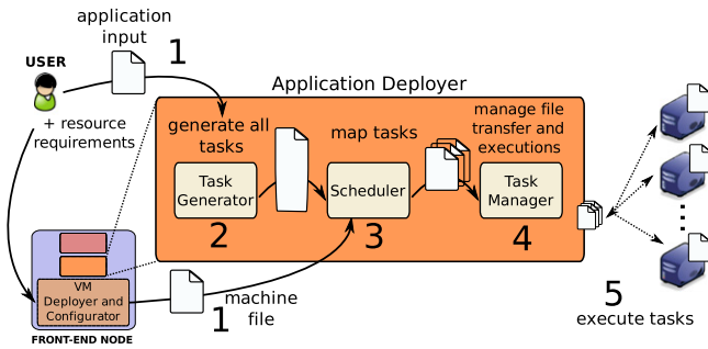
Fig. 4. Application deployer.
