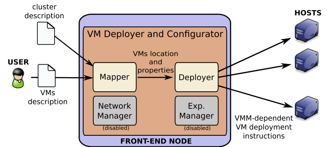
Fig. 5. AEF framework.
