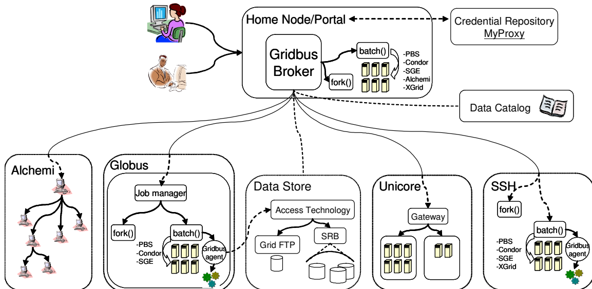
Figure 1 : Broker Block Diagram.
